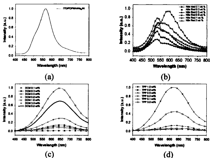
FIGURE 1 The EL spectra of ITO/dye doped PDPMA/Alq 3 /Al :
